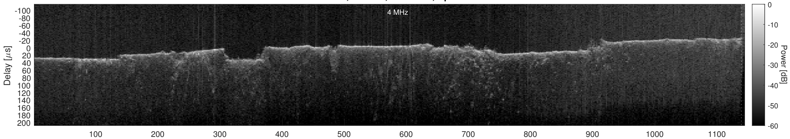
Orbit 11185, Cluttergram
