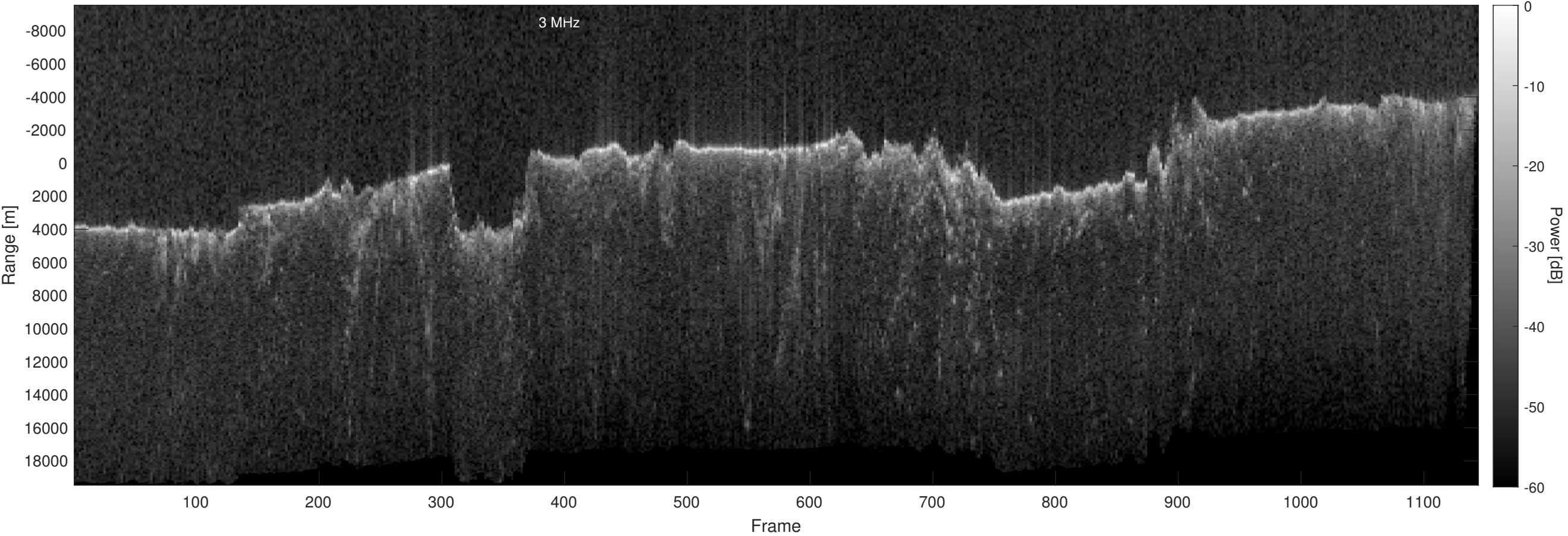
Orbit 11185, Optimized, Window, Depth-Corrected, Channel 2
