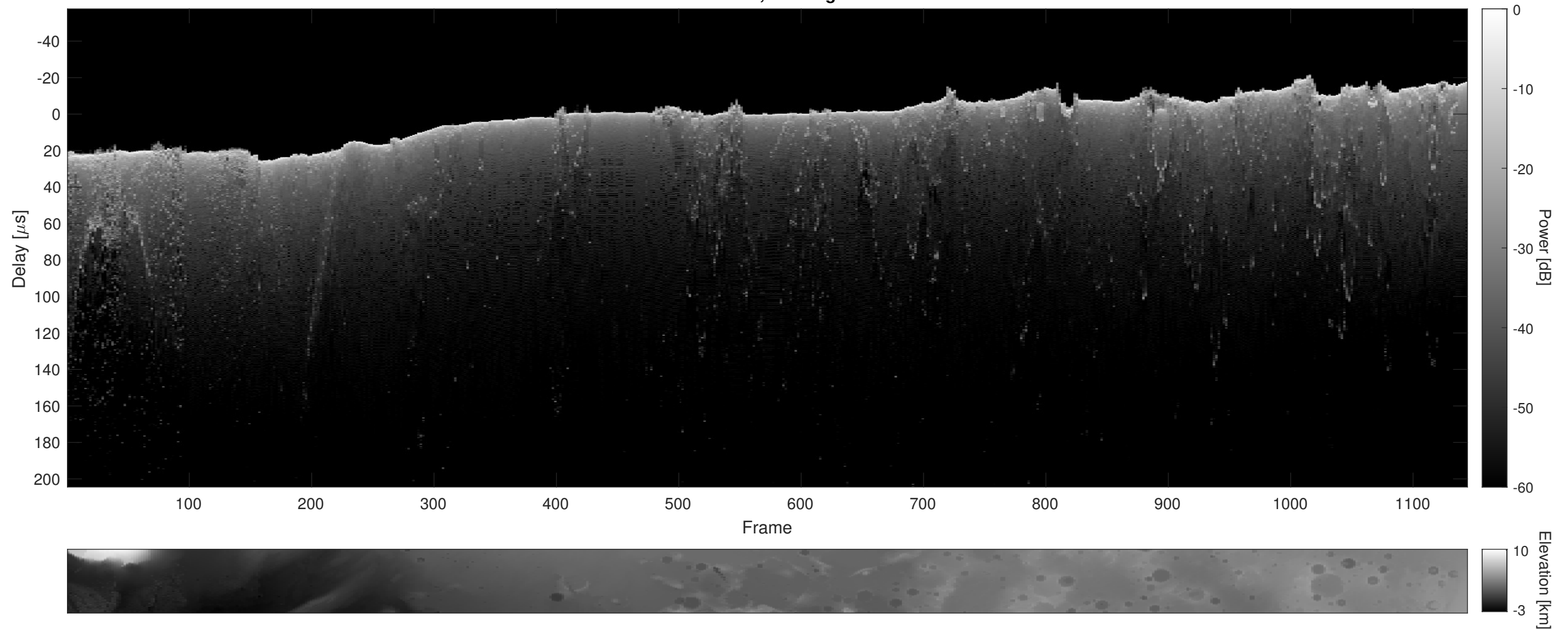
Orbit 11186, Cluttergram
