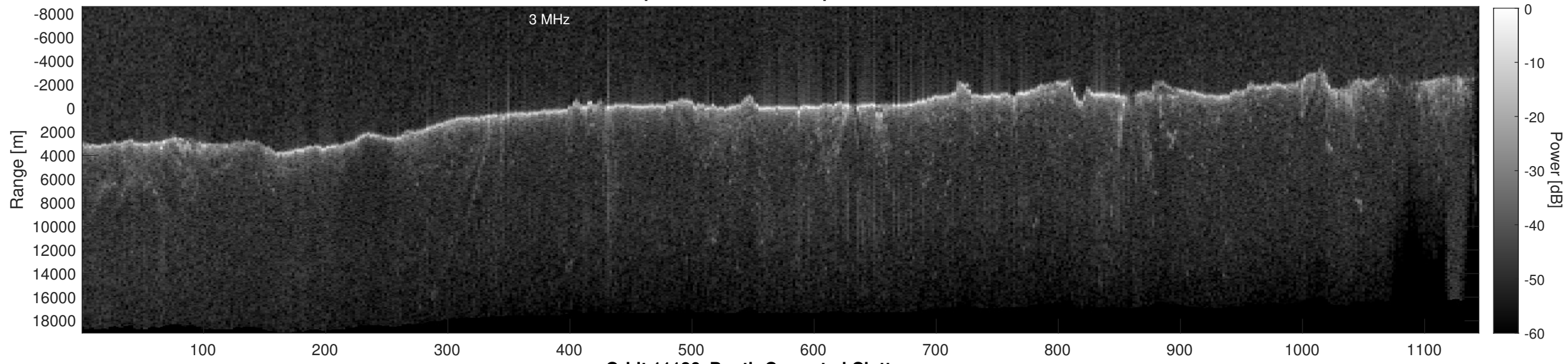
Orbit 11186, Depth-Corrected Cluttergram
