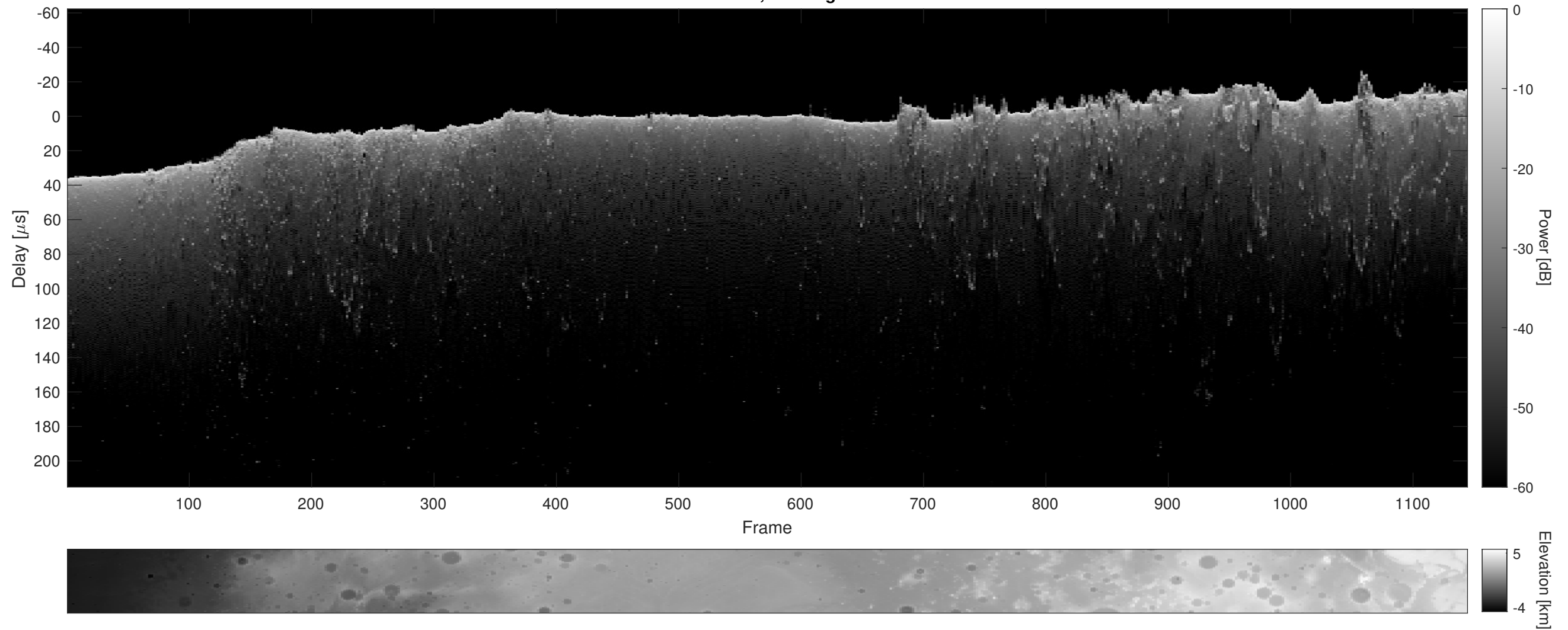
Orbit 11187, Cluttergram
