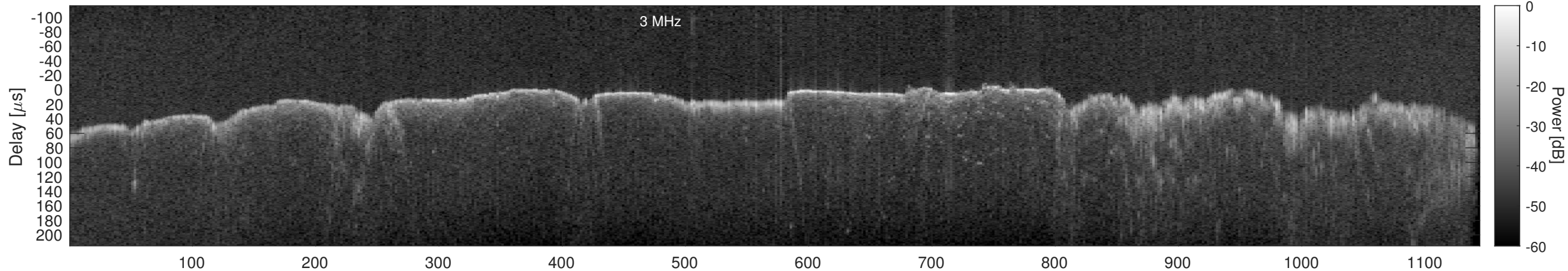
Orbit 11187, Window, Channel 2, Chapman
