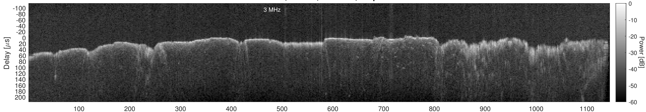
Orbit 11187, Window, Channel 2, Optimized
