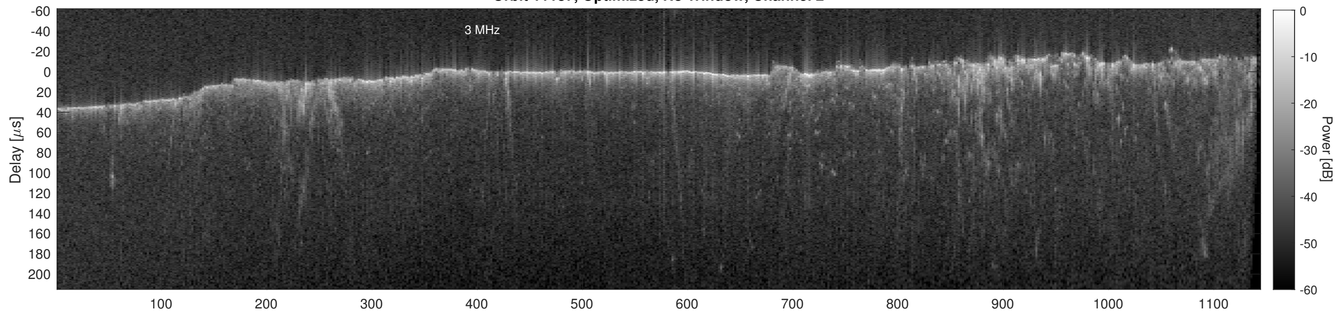
Orbit 11187, Cluttergram
