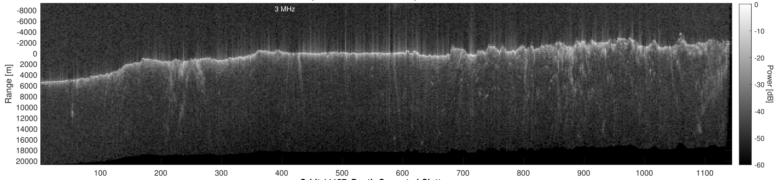
Orbit 11187, Depth-Corrected Cluttergram
