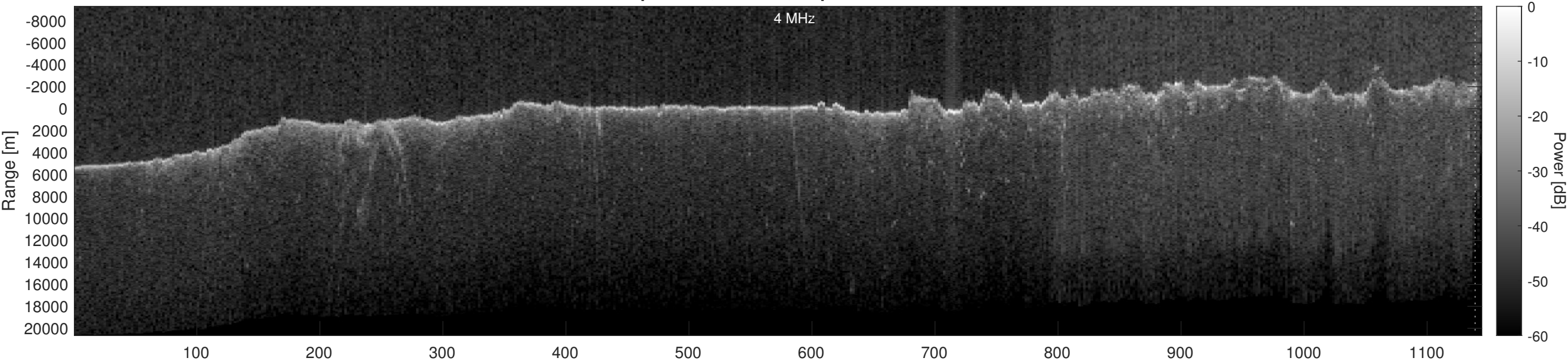
Orbit 11187, Optimized, Window, Depth-Corrected, Channel 2
