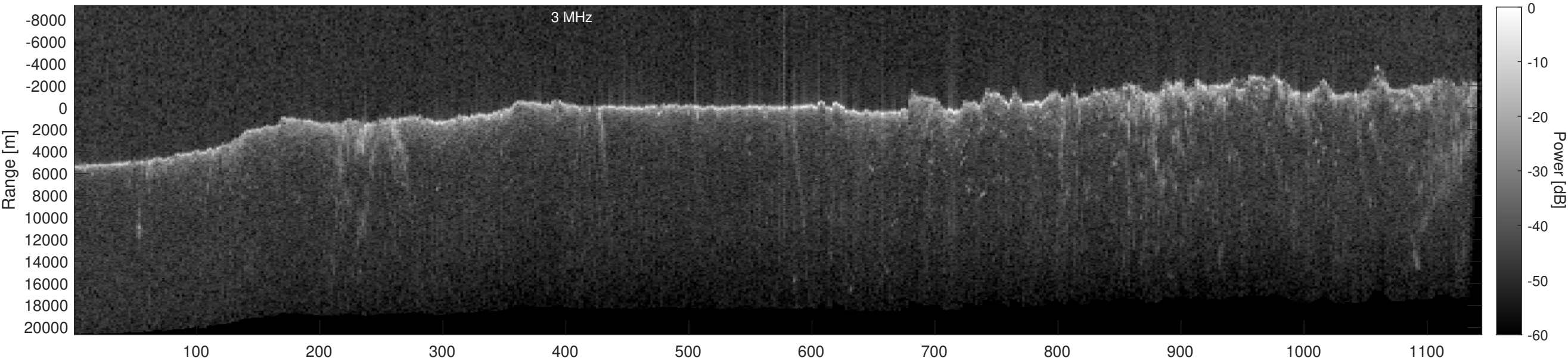
Orbit 11187, Depth-Corrected Cluttergram
