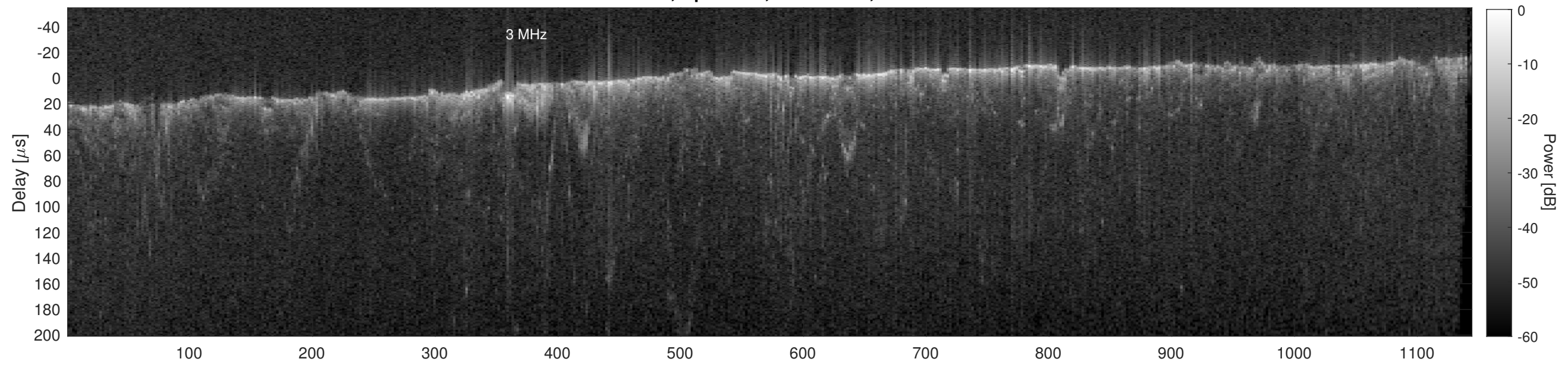
Orbit 11188, Cluttergram
