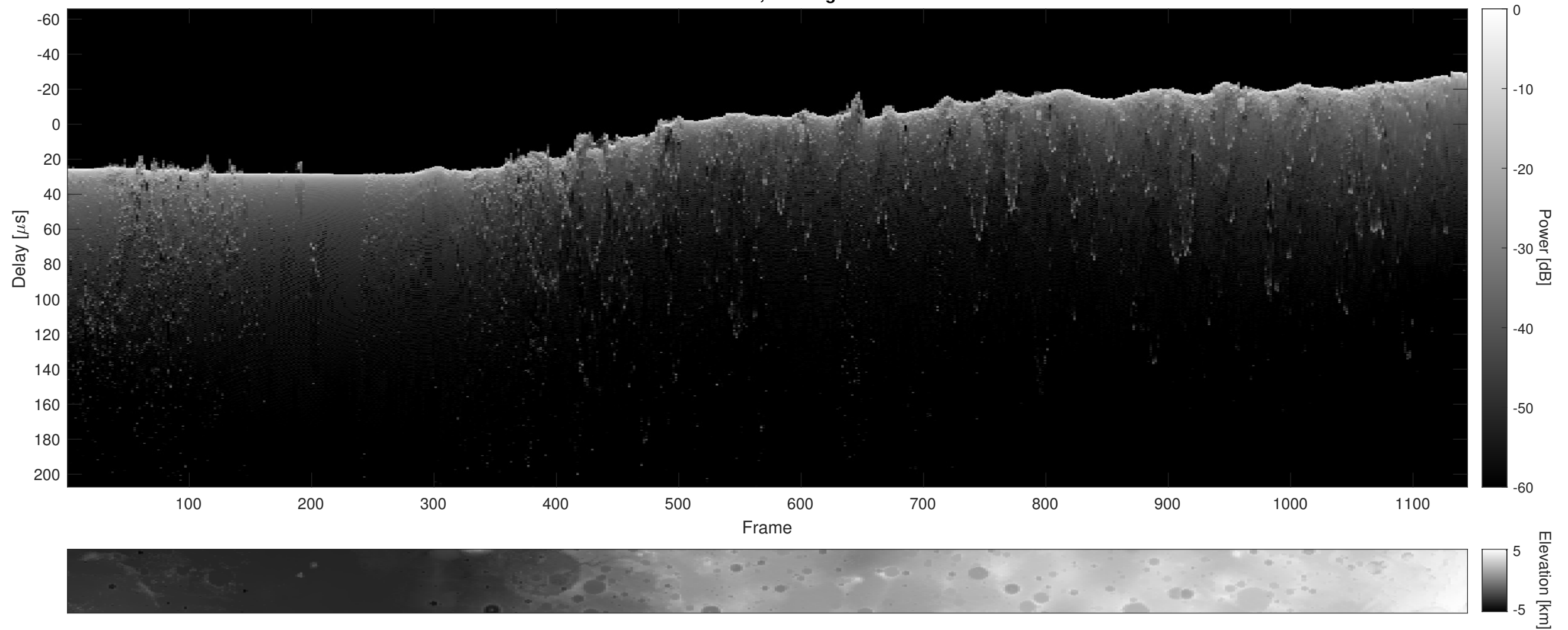
Orbit 11190, Cluttergram
