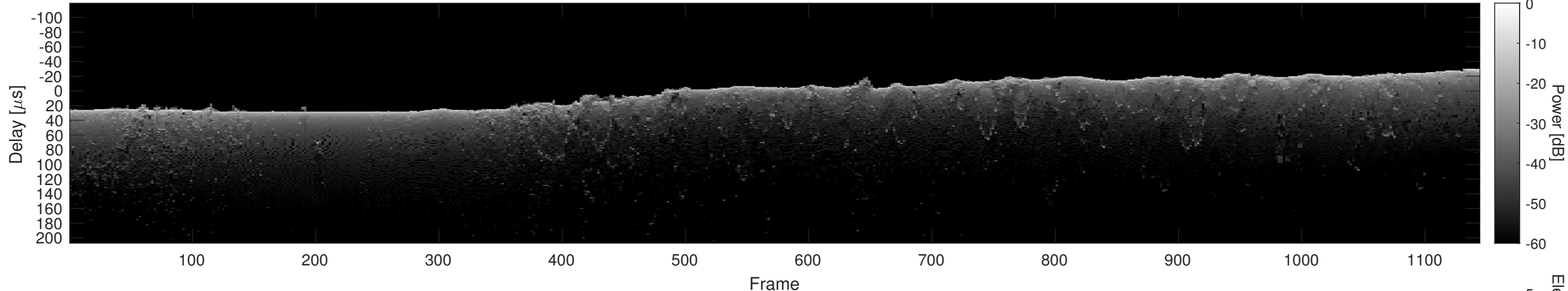
Orbit 11190, Cluttergram
