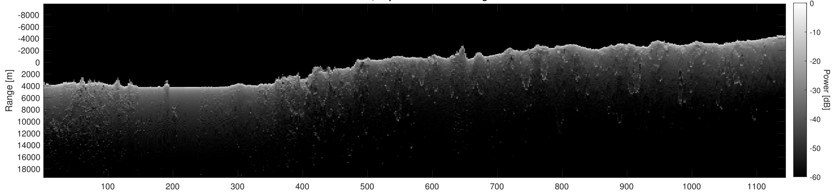
Orbit 11190, Depth-Corrected Cluttergram
