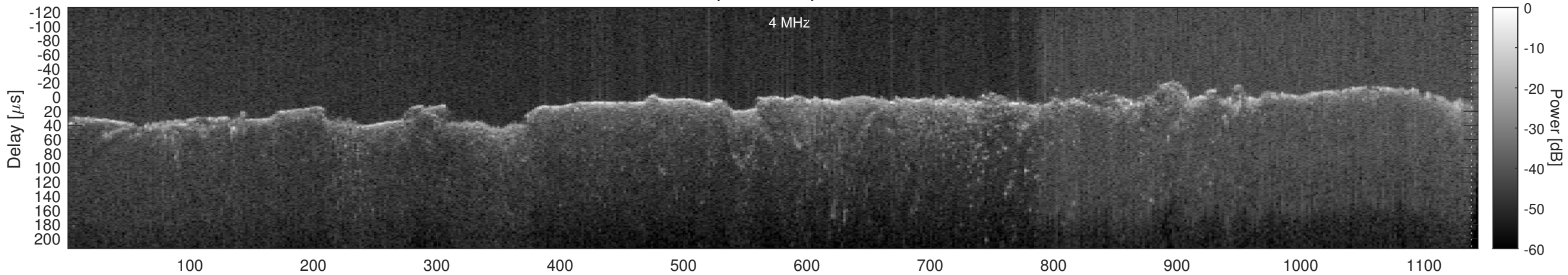
Orbit 11192, Window, Channel 1, Chapman
