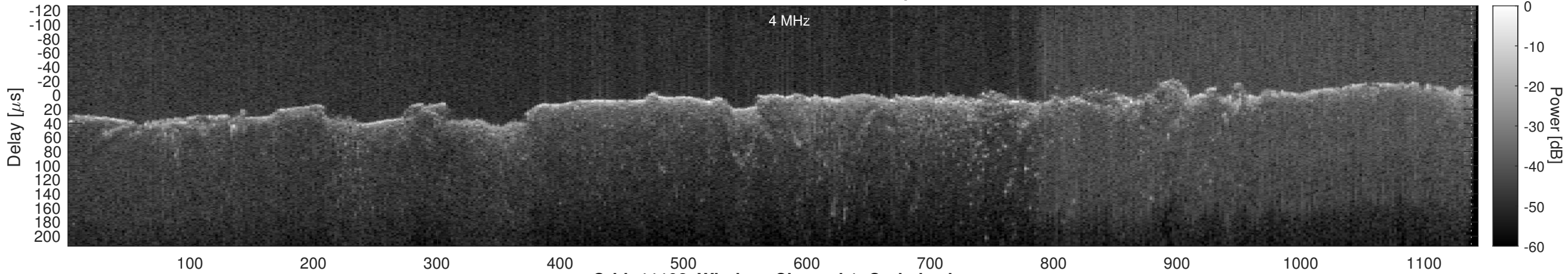
Orbit 11192, Window, Channel 1, Optimized
