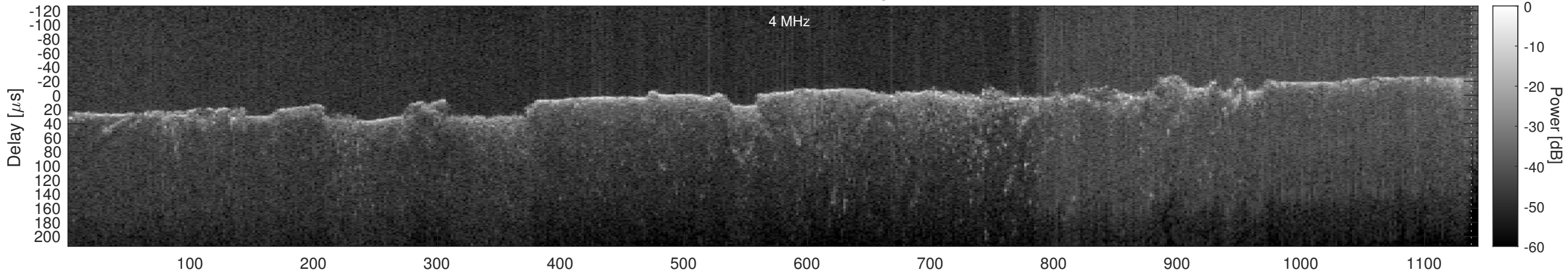
Orbit 11192, Cluttergram
