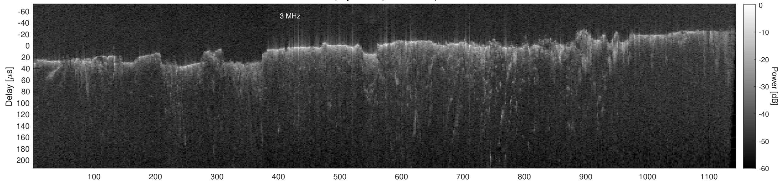
Orbit 11192, Cluttergram
