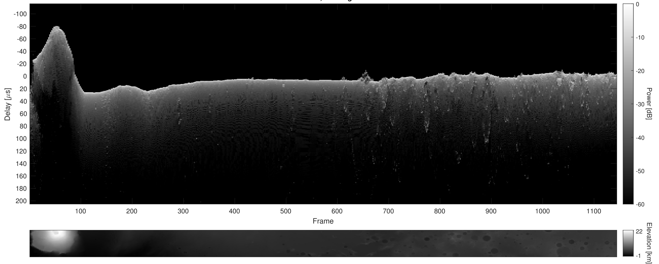
Orbit 11193, Cluttergram
