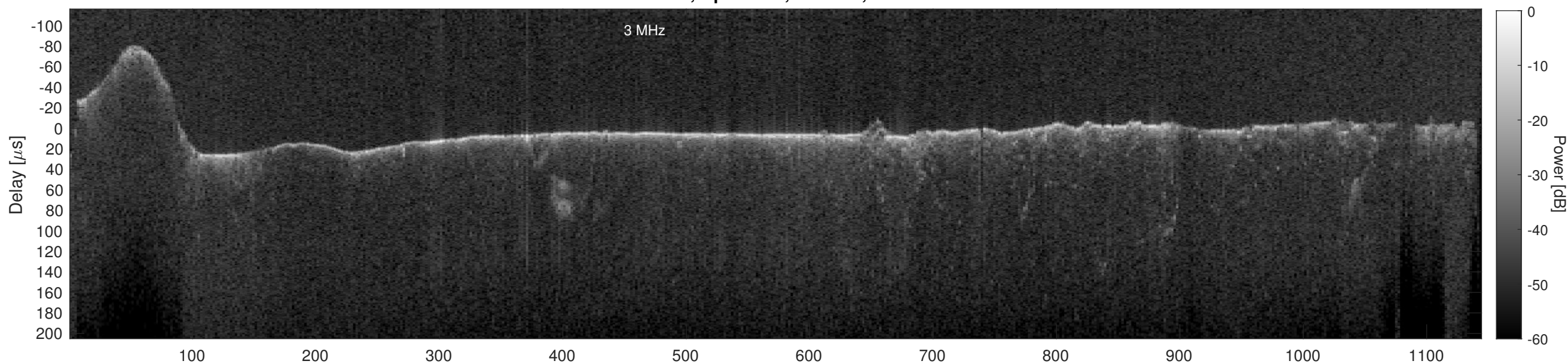
Orbit 11193, Cluttergram
