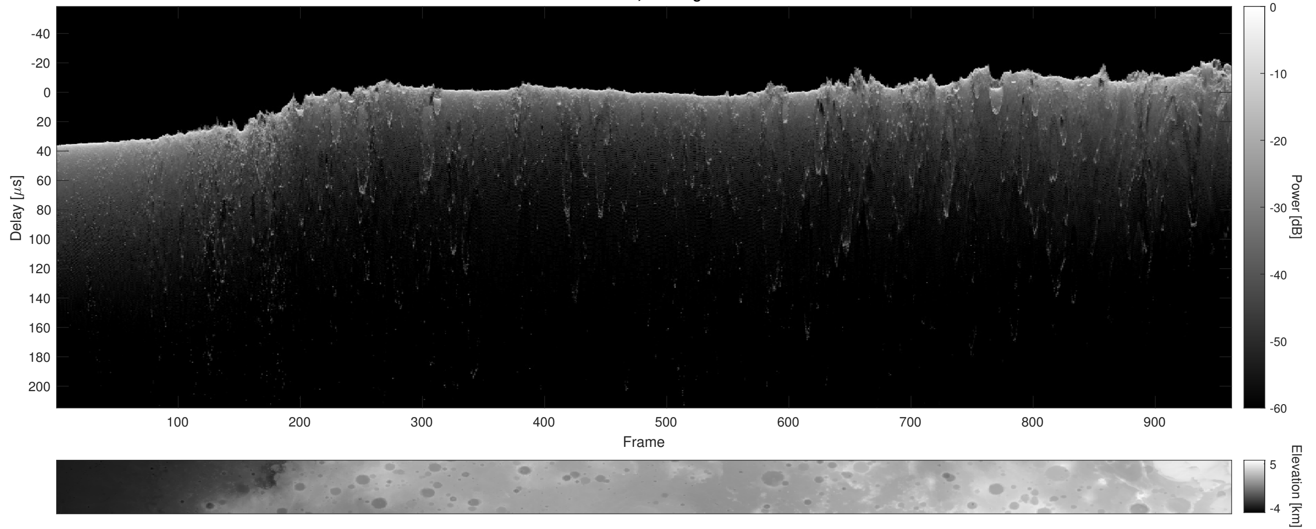
Orbit 11194, Cluttergram
