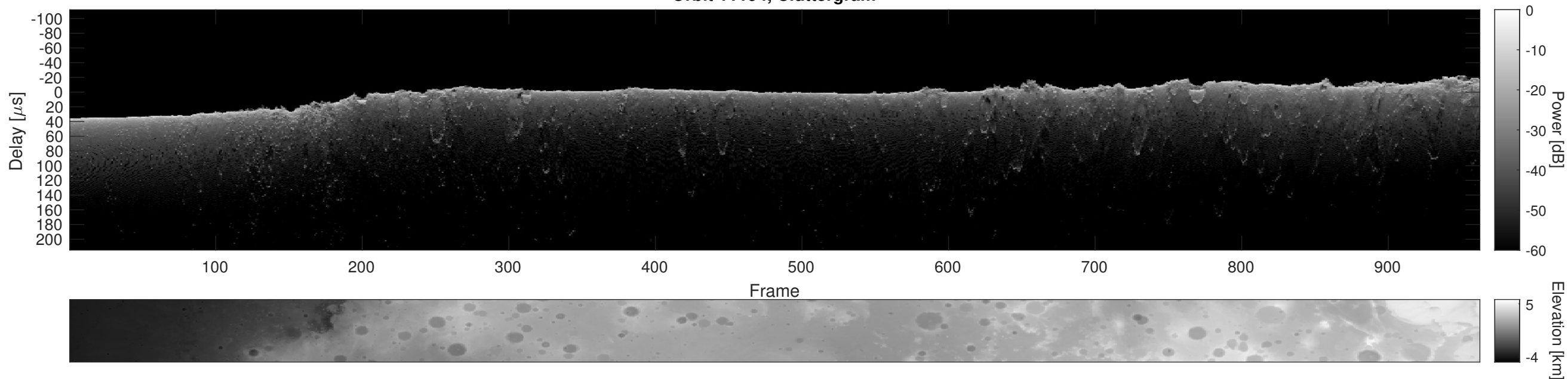
Orbit 11194, Cluttergram
