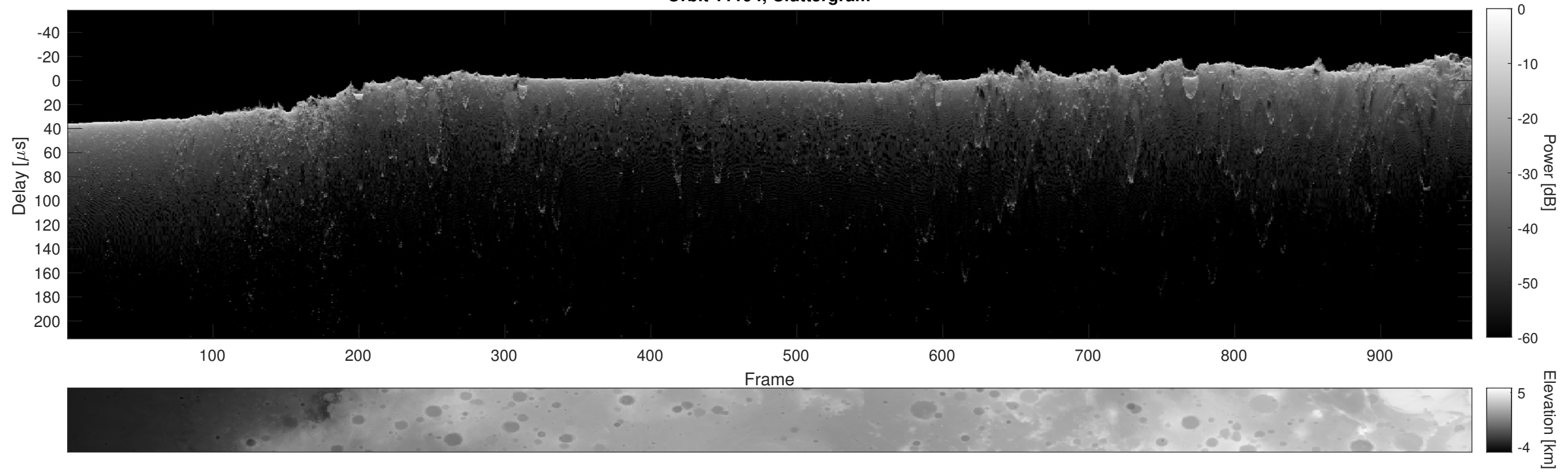
Orbit 11194, Cluttergram
