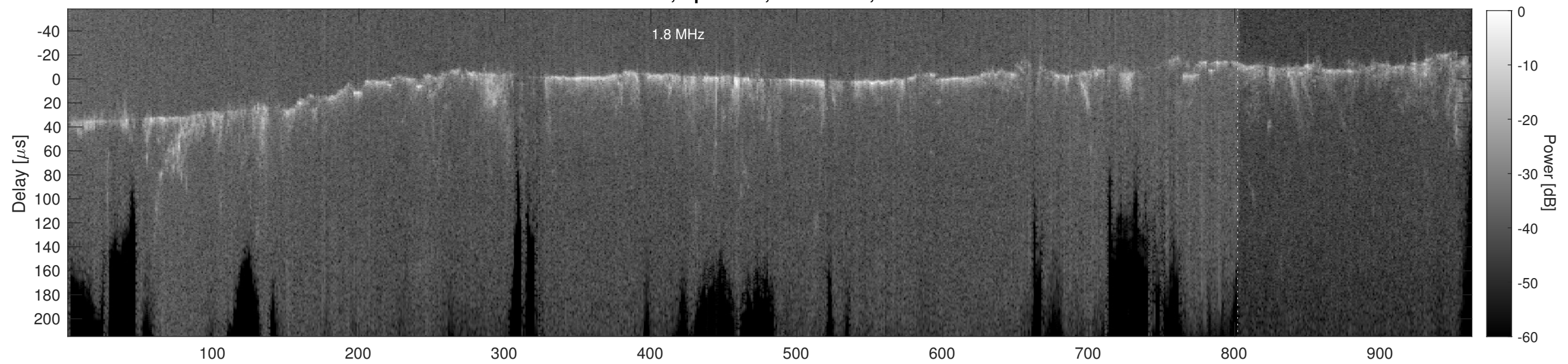
Orbit 11194, Cluttergram
