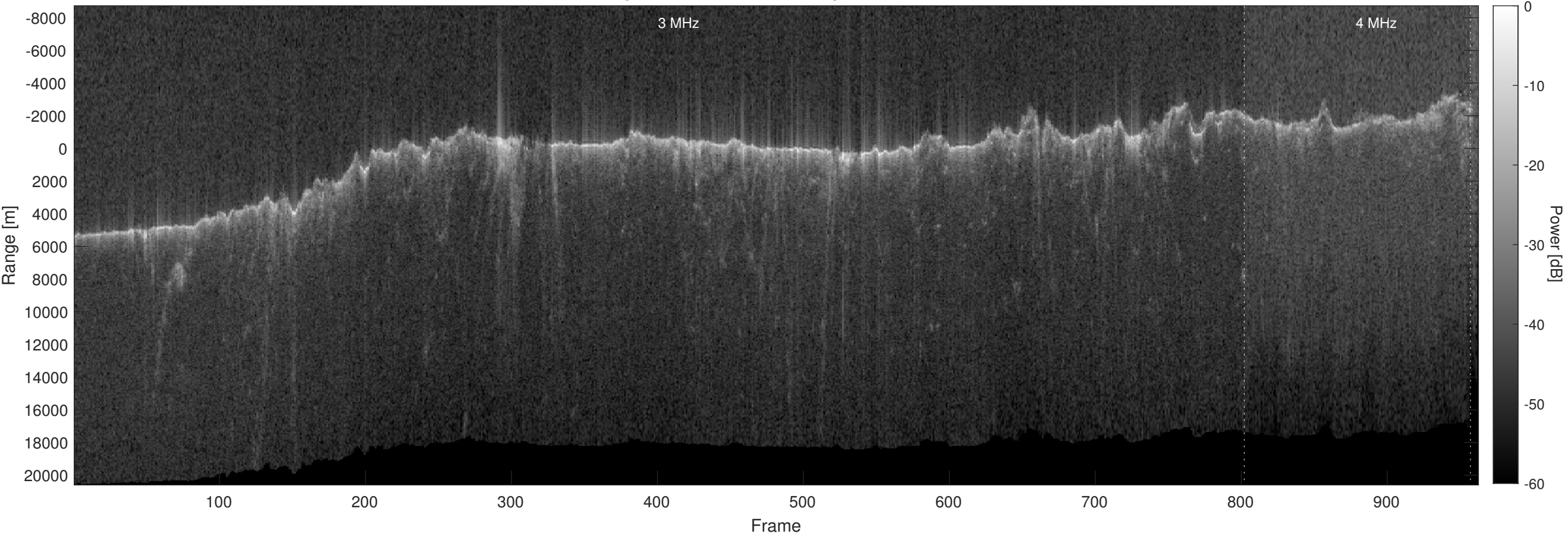
Orbit 11194, Optimized, No Window, Depth-Corrected, Channel 2
