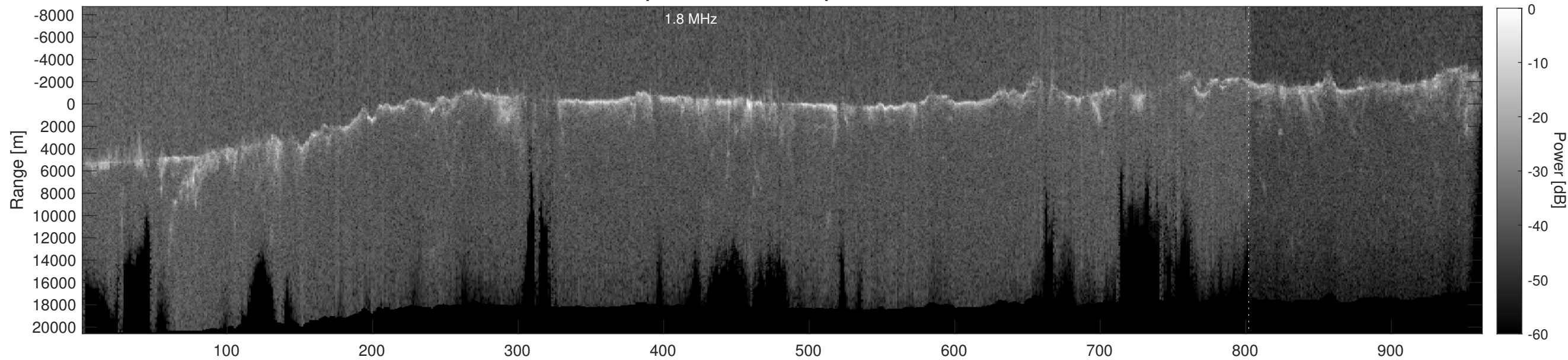
Orbit 11194, Depth-Corrected Cluttergram
