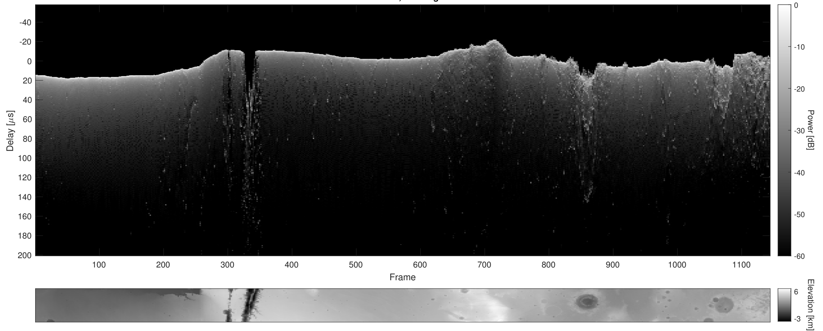
Orbit 11196, Cluttergram
