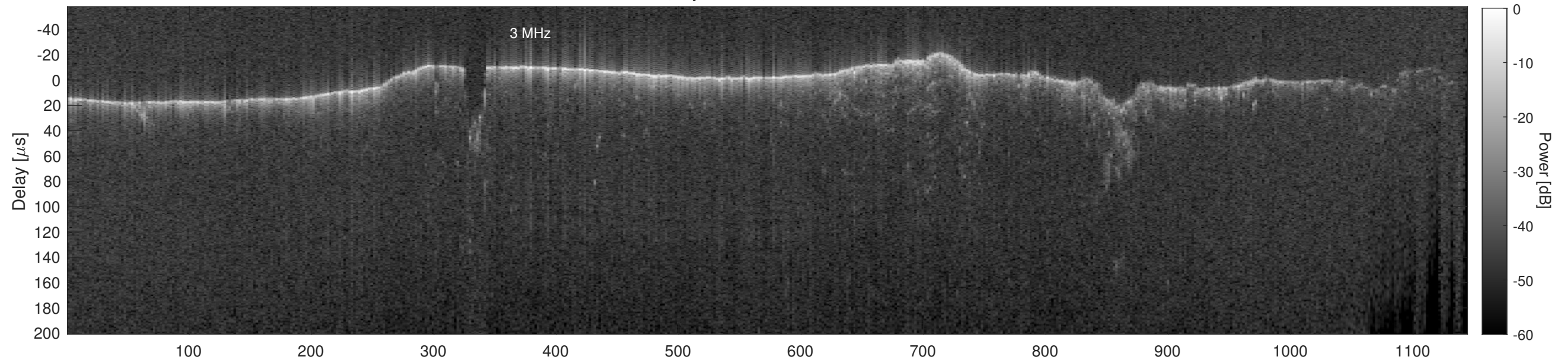
Orbit 11196, Cluttergram
