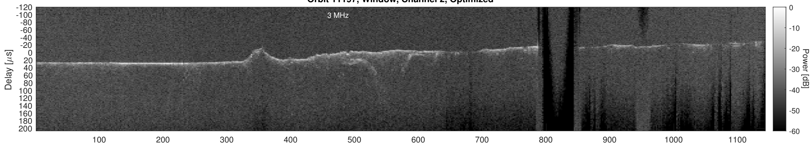
Orbit 11197, Cluttergram
