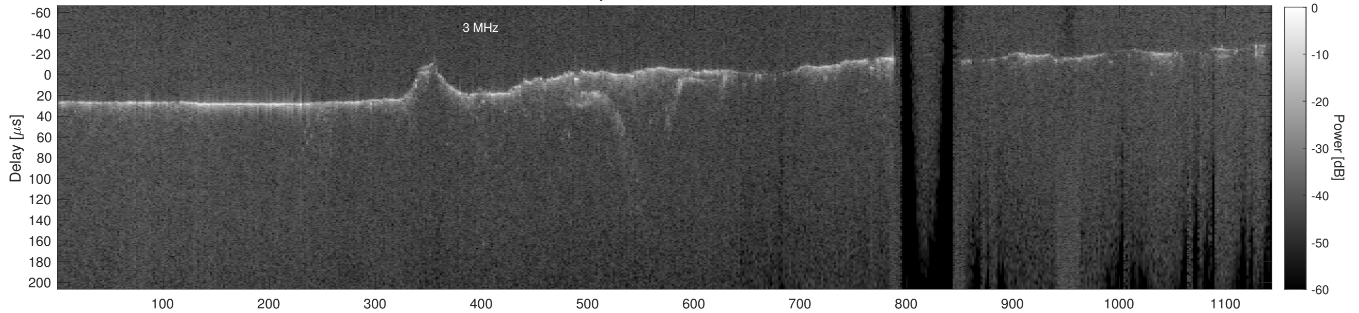
Orbit 11197, Cluttergram
