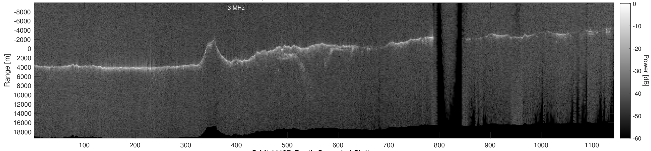
Orbit 11197, Depth-Corrected Cluttergram
