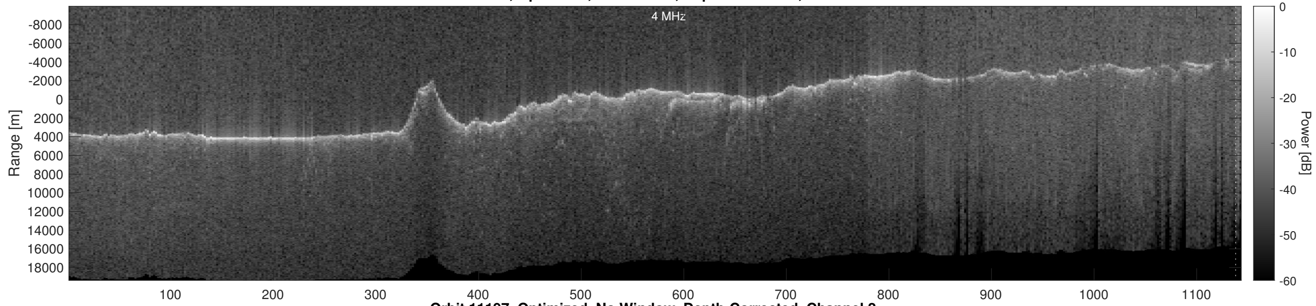
Orbit 11197, Optimized, No Window, Depth-Corrected, Channel 2
