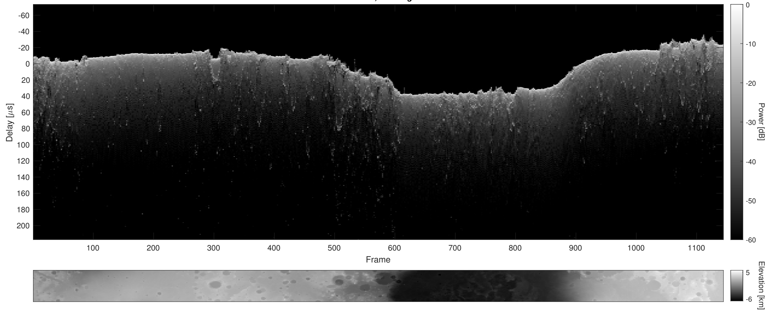
Orbit 11198, Cluttergram
