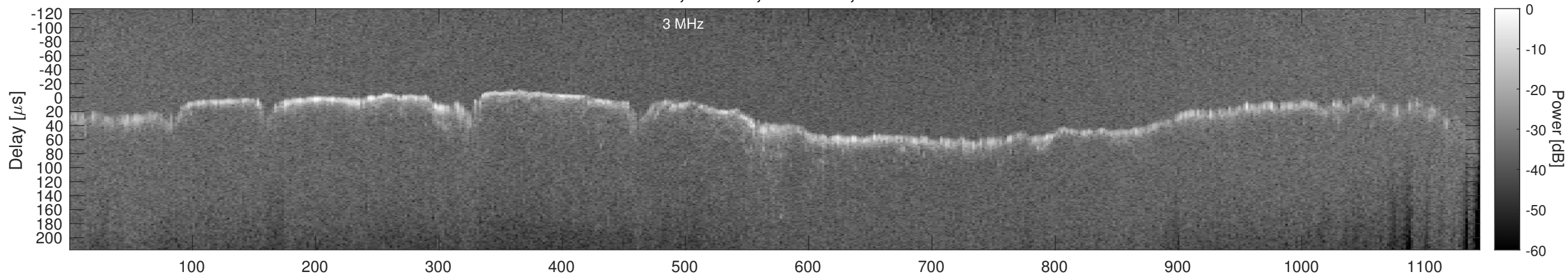
Orbit 11198, Window, Channel 2, Chapman
