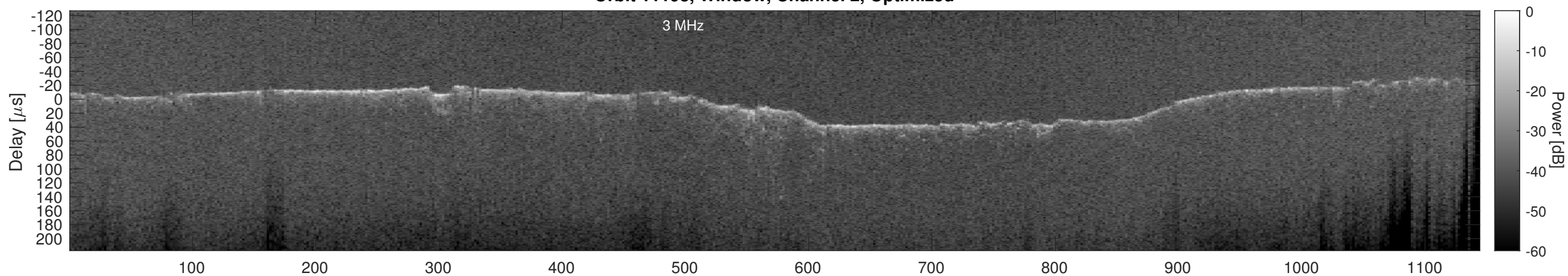
Orbit 11198, Cluttergram
