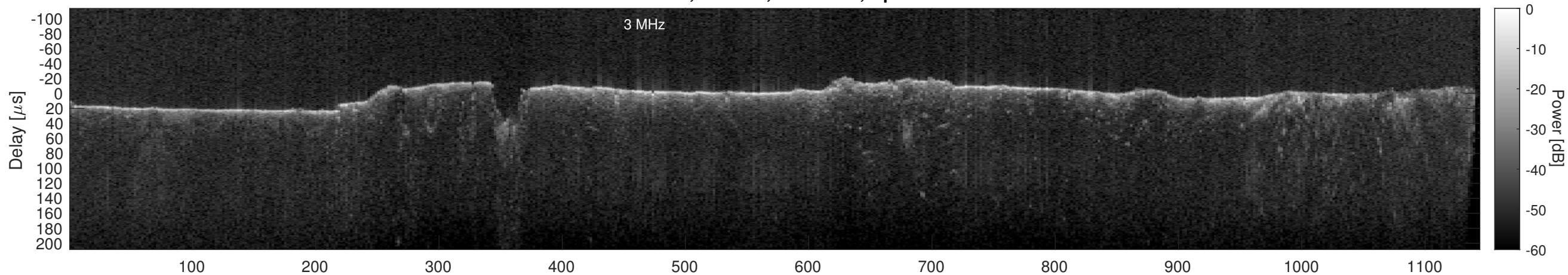
Orbit 11203, Cluttergram
