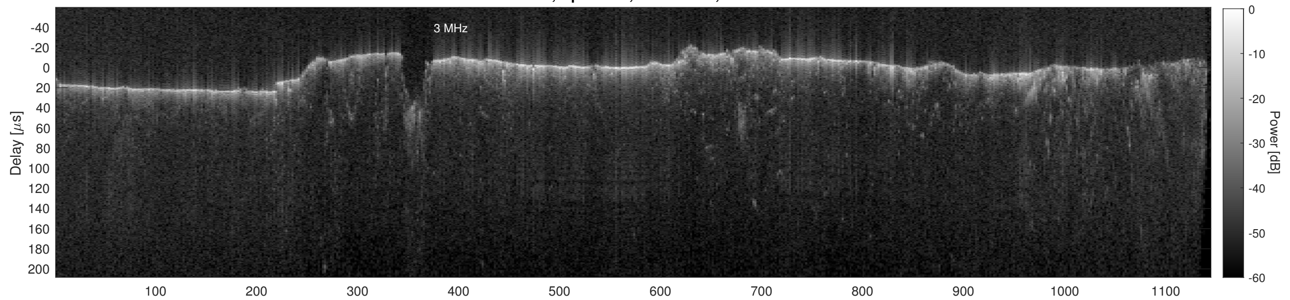
Orbit 11203, Cluttergram
