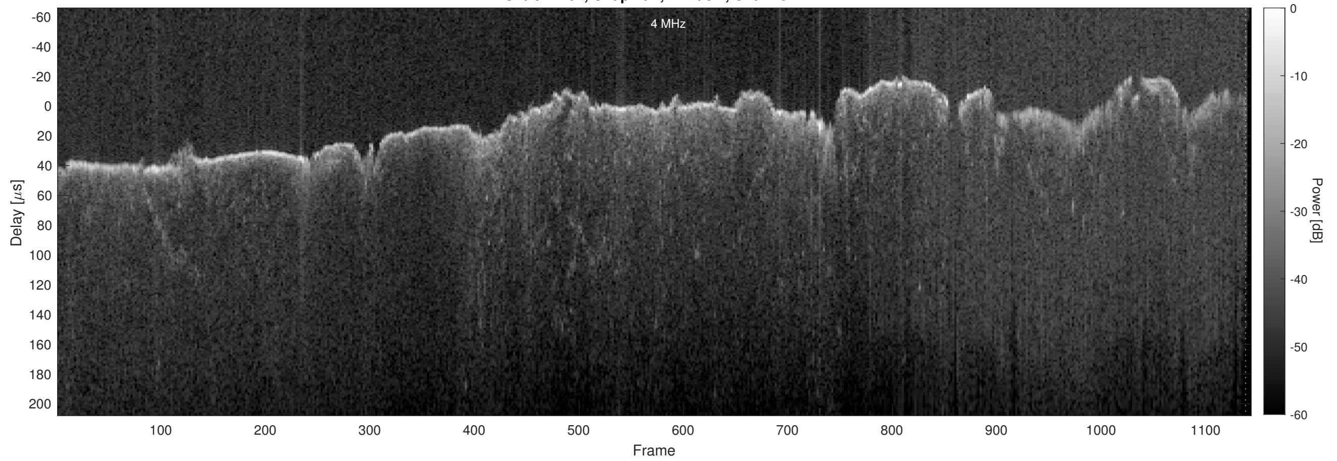
Orbit 11204, Chapman, Window, Channel 2
