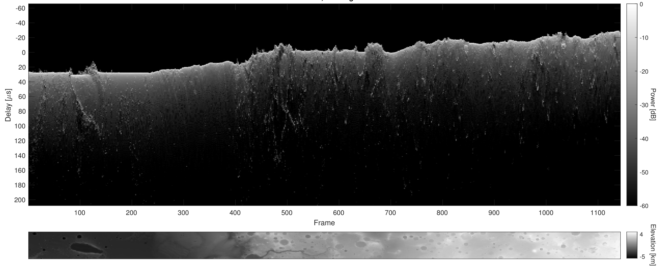
Orbit 11204, Cluttergram
