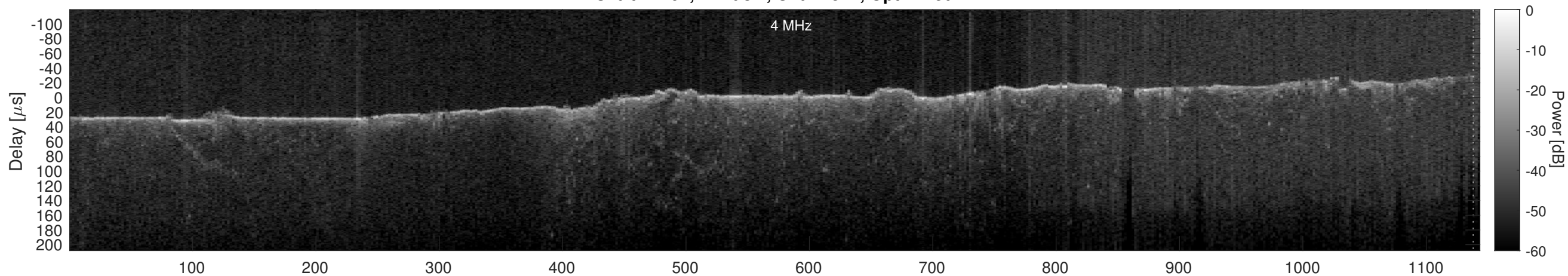
Orbit 11204, Cluttergram
