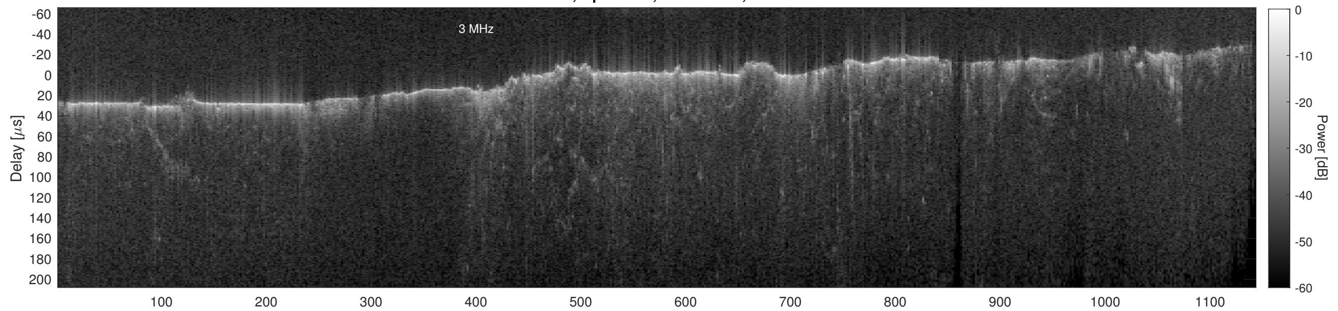
Orbit 11204, Cluttergram
