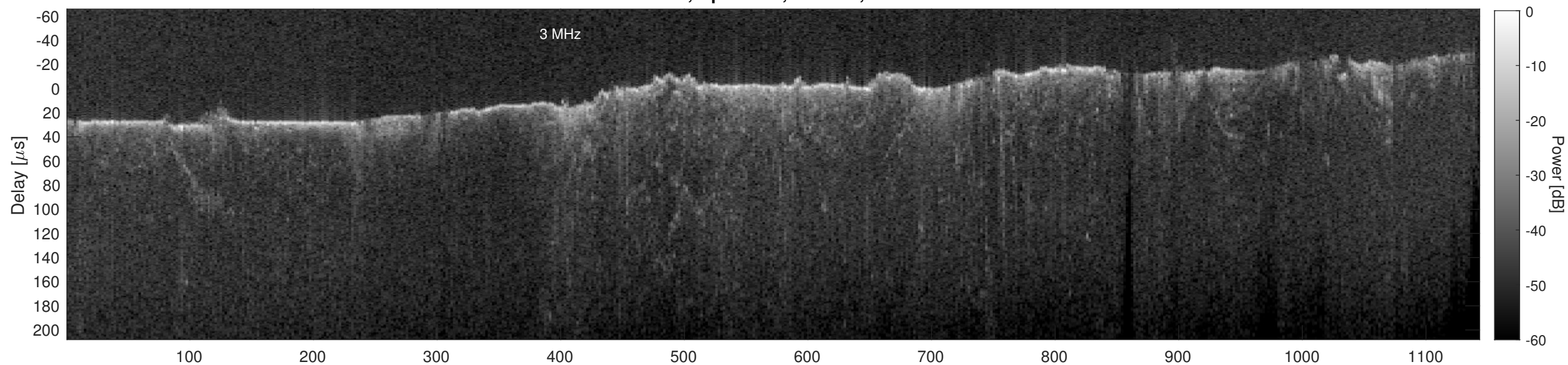
Orbit 11204, Cluttergram
