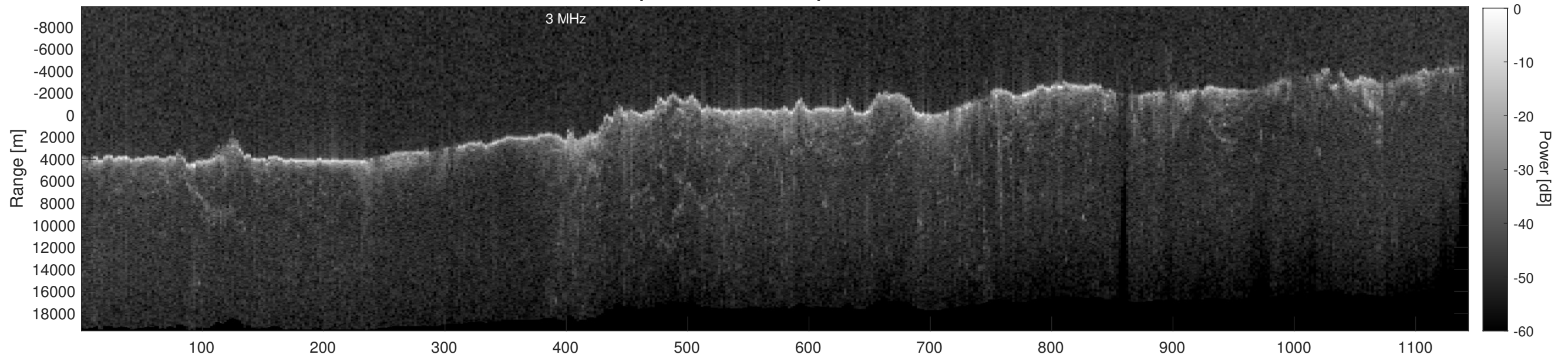
Orbit 11204, Depth-Corrected Cluttergram
