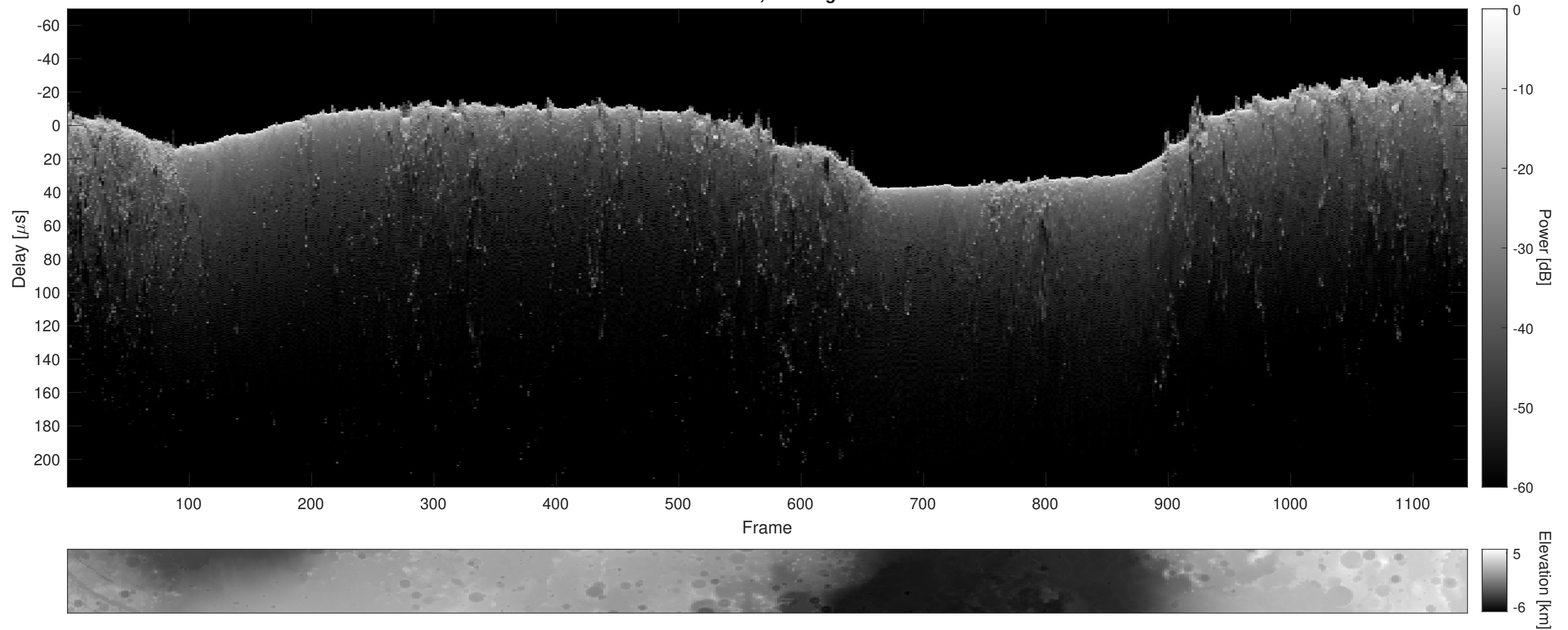
Orbit 11205, Cluttergram
