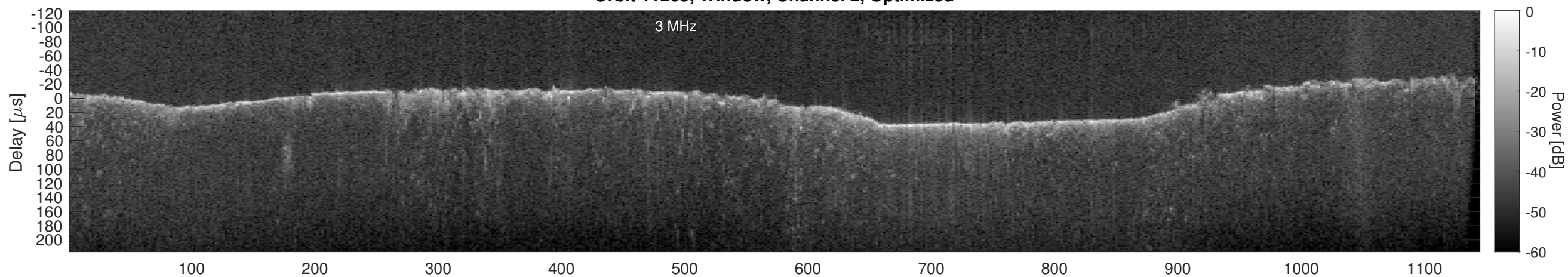
Orbit 11205, Cluttergram
