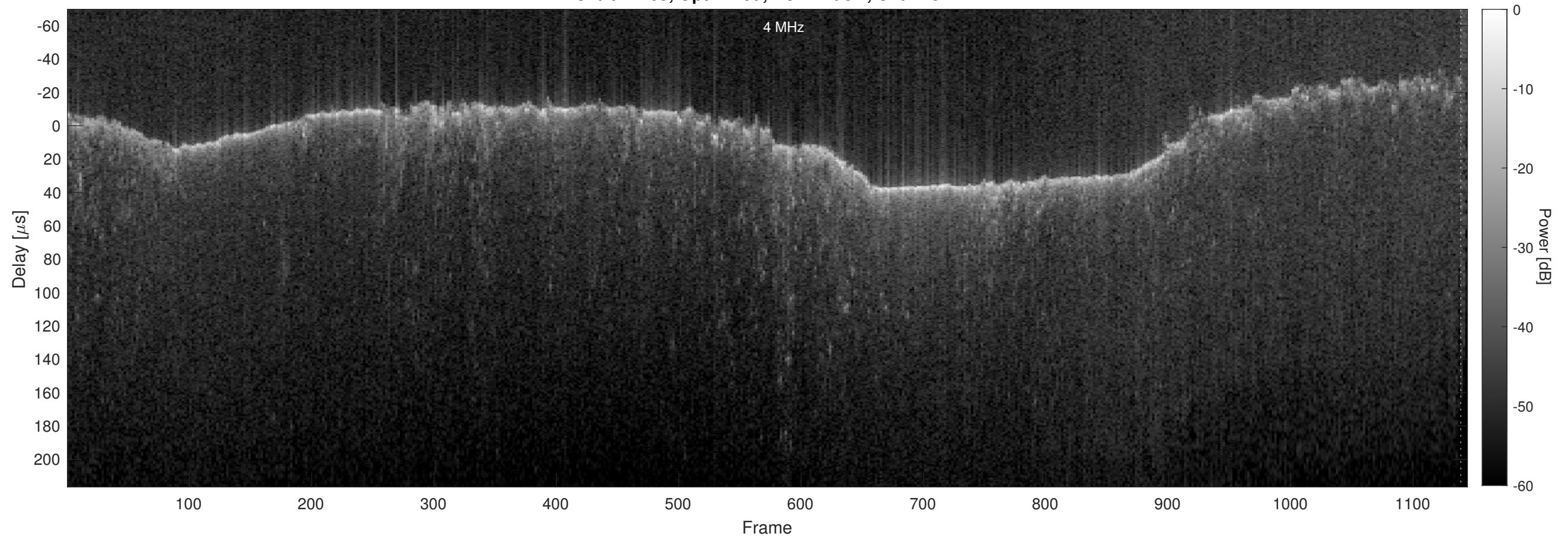
Orbit 11205, Optimized, No Window, Channel 2
