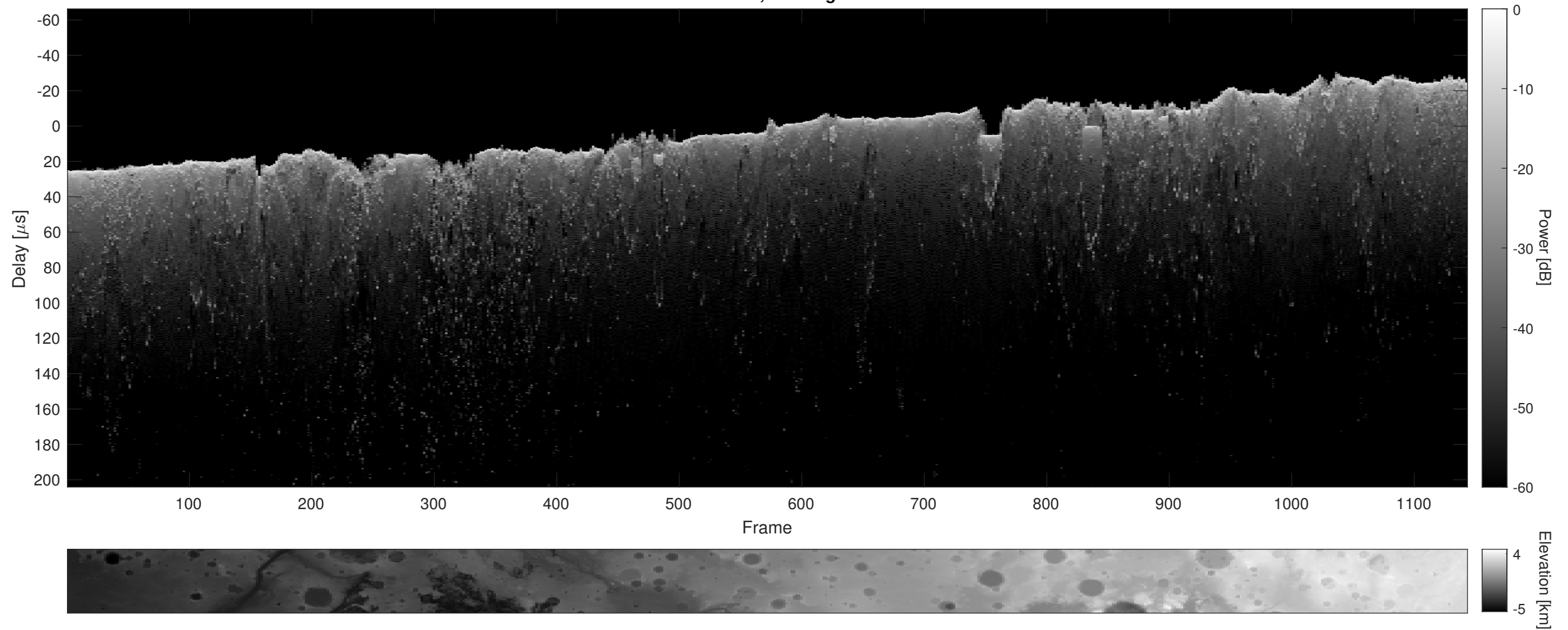
Orbit 11206, Cluttergram
