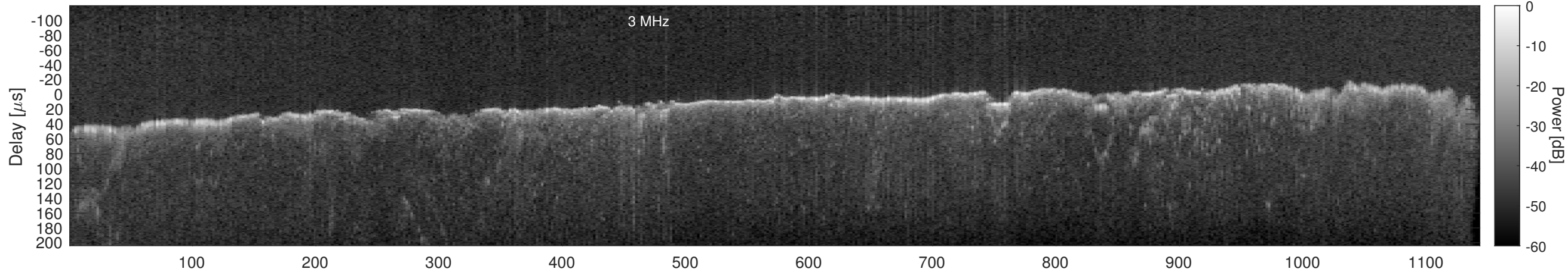
Orbit 11206, Window, Channel 2, Chapman
