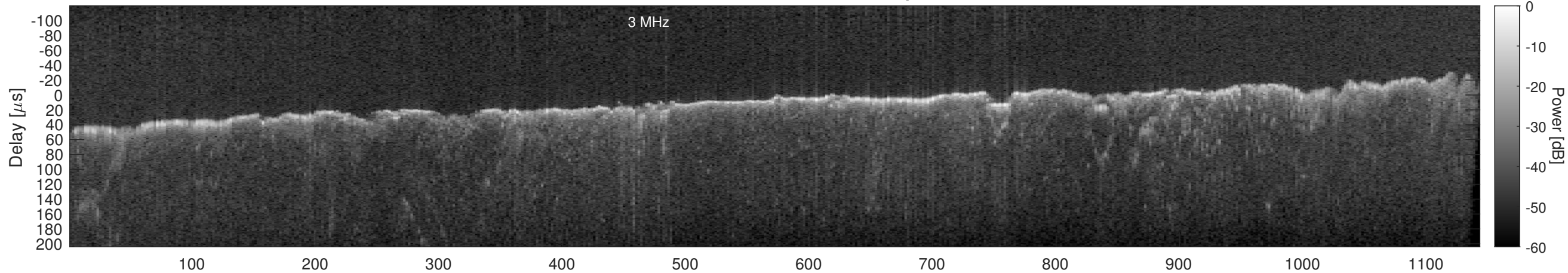
Orbit 11206, Window, Channel 2, Optimized
