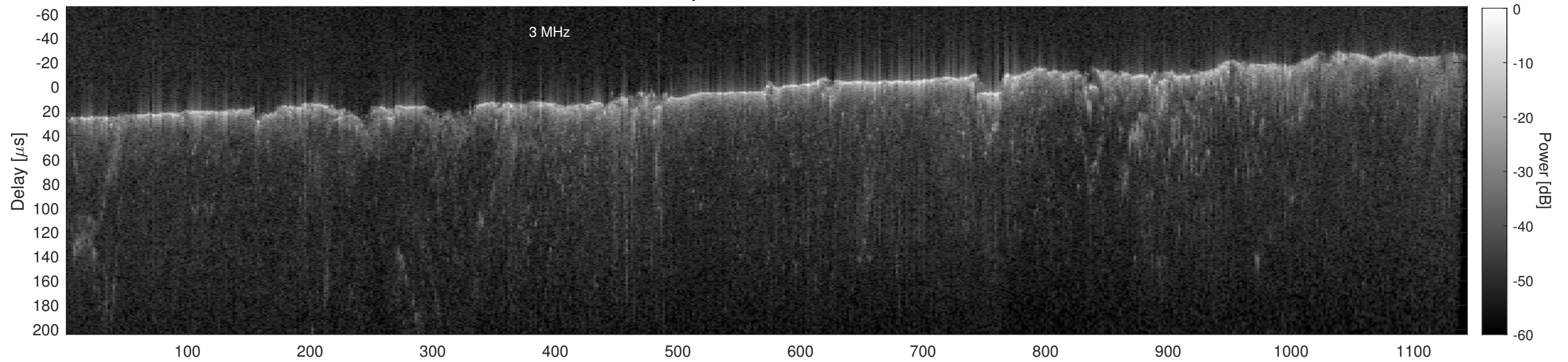
Orbit 11206, Cluttergram
