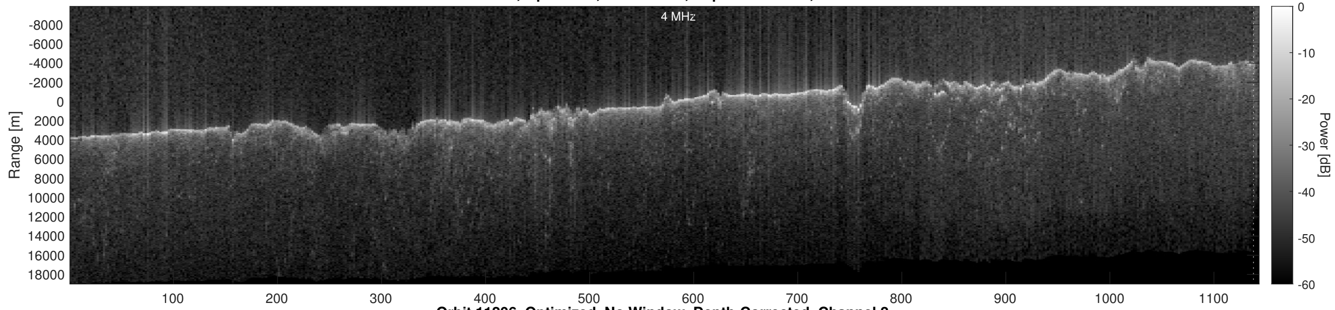
Orbit 11206, Optimized, No Window, Depth-Corrected, Channel 2
