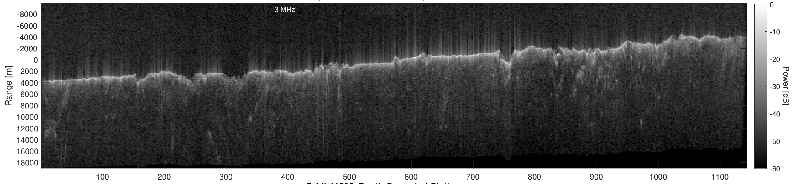
Orbit 11206, Depth-Corrected Cluttergram
