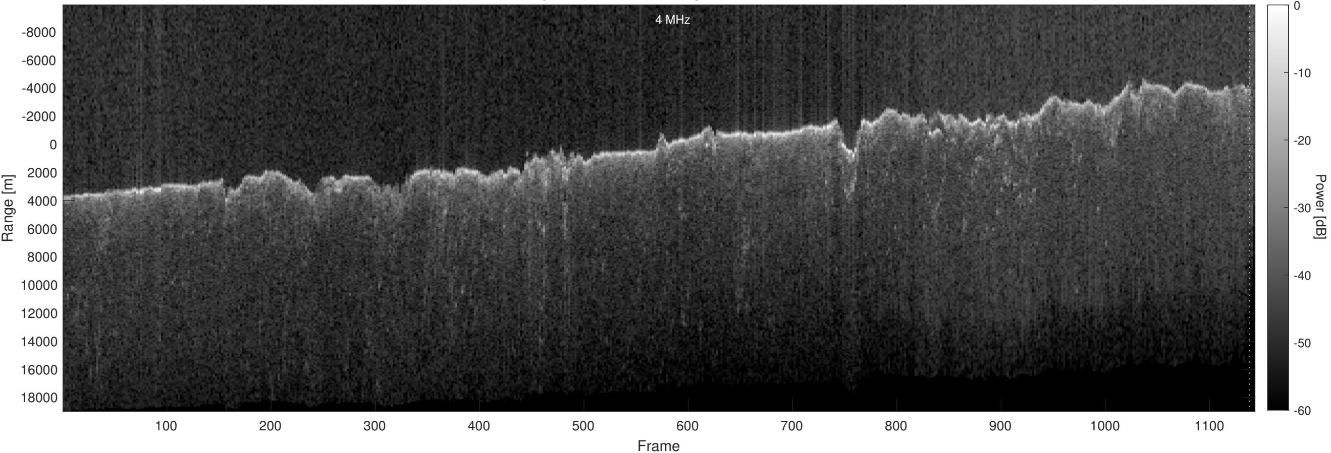
Orbit 11206, Optimized, Window, Depth-Corrected, Channel 2
