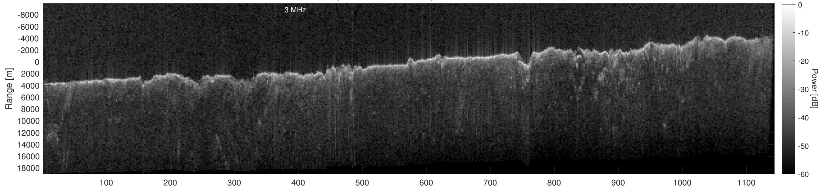
Orbit 11206, Depth-Corrected Cluttergram
