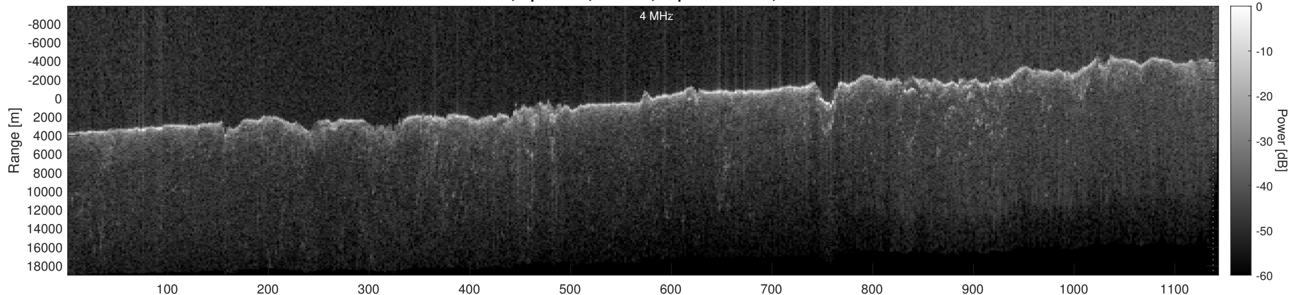
Orbit 11206, Optimized, Window, Depth-Corrected, Channel 2
