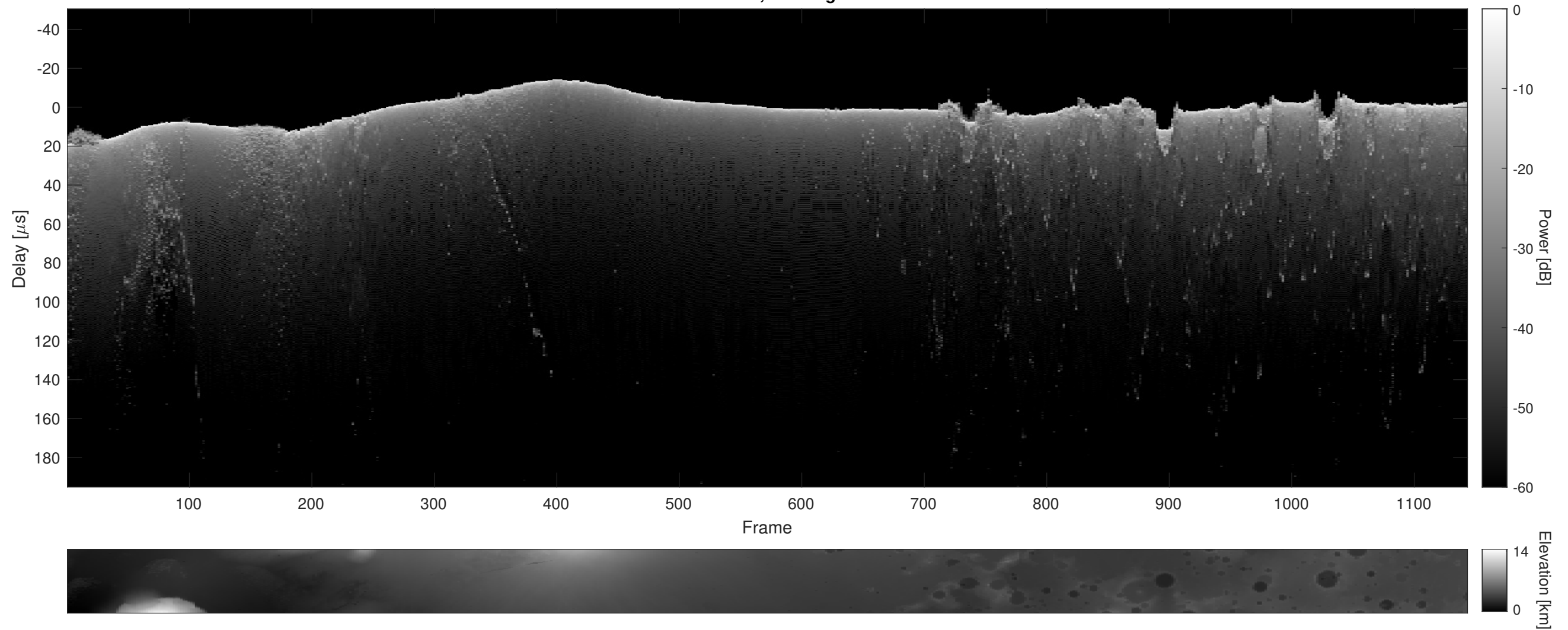
Orbit 11207, Cluttergram
