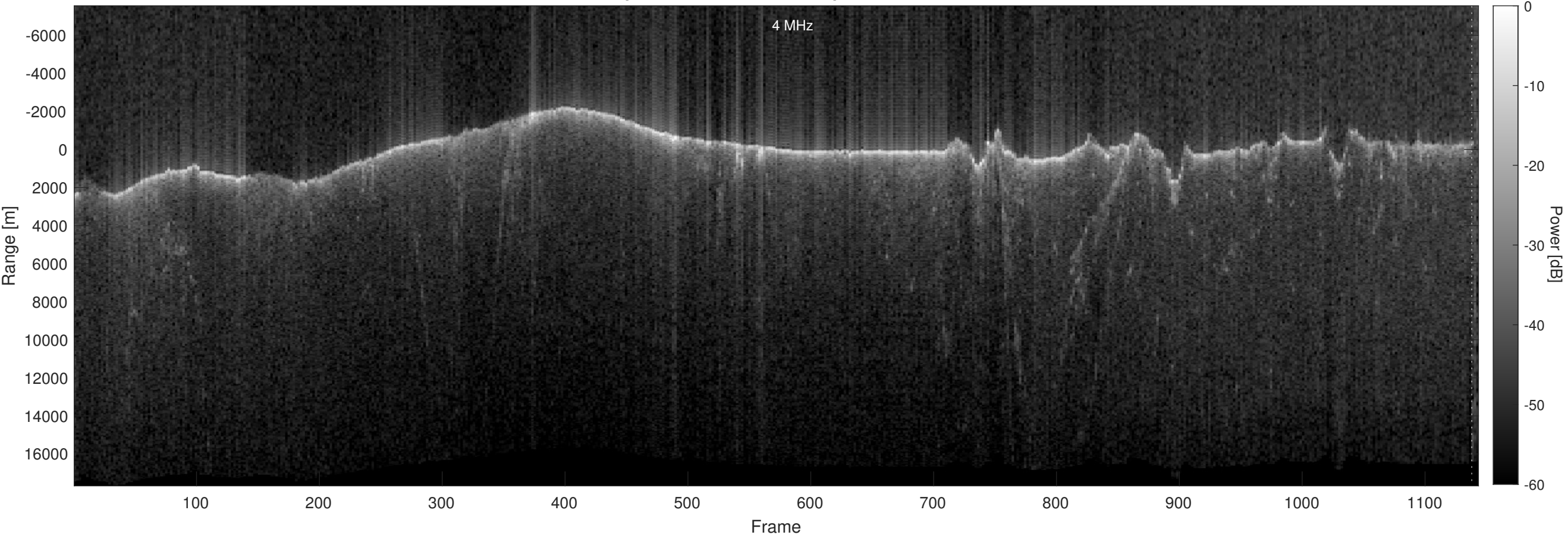
Orbit 11207, Optimized, No Window, Depth-Corrected, Channel 2
