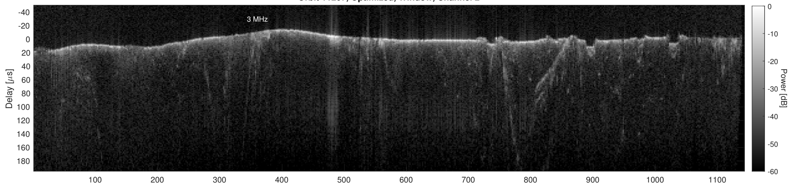
Orbit 11207, Cluttergram
