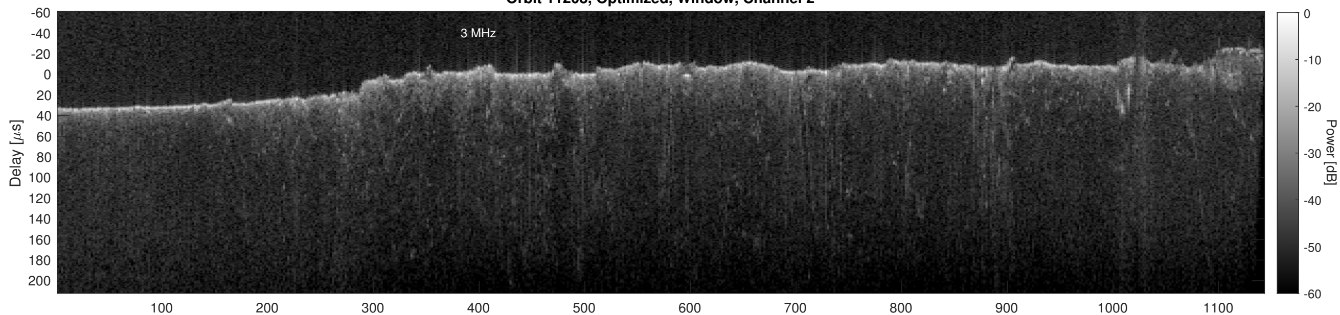
Orbit 11208, Cluttergram
